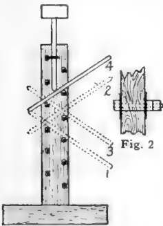
This Jack Will Not Kick or Cut Into the Object Lifted
